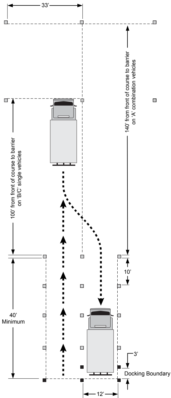
Figure 12.2 Offset backing to the right
